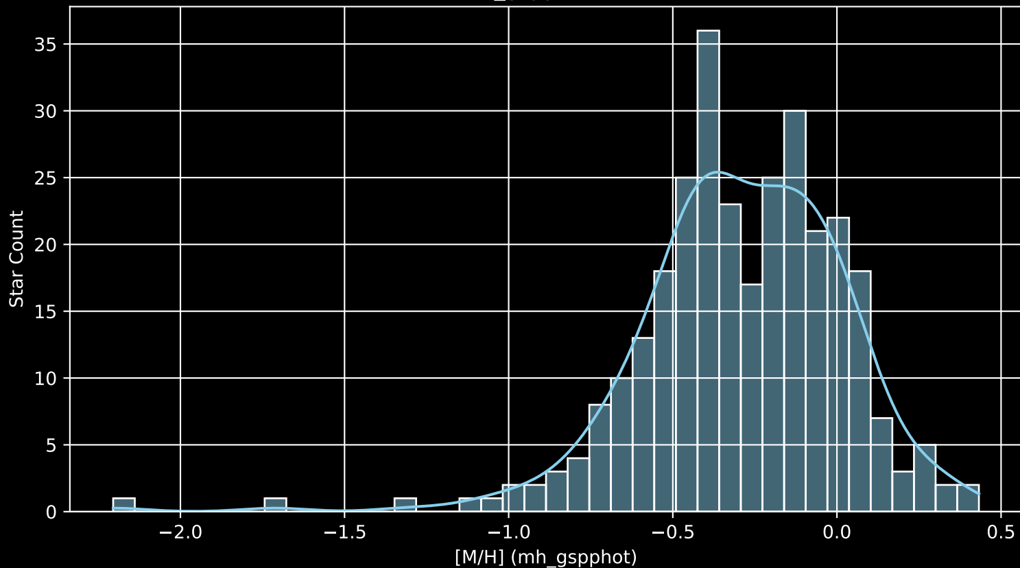
GALAH DR4 Field: [7045] [M/H] (mh_gspphot) (n= 301)
