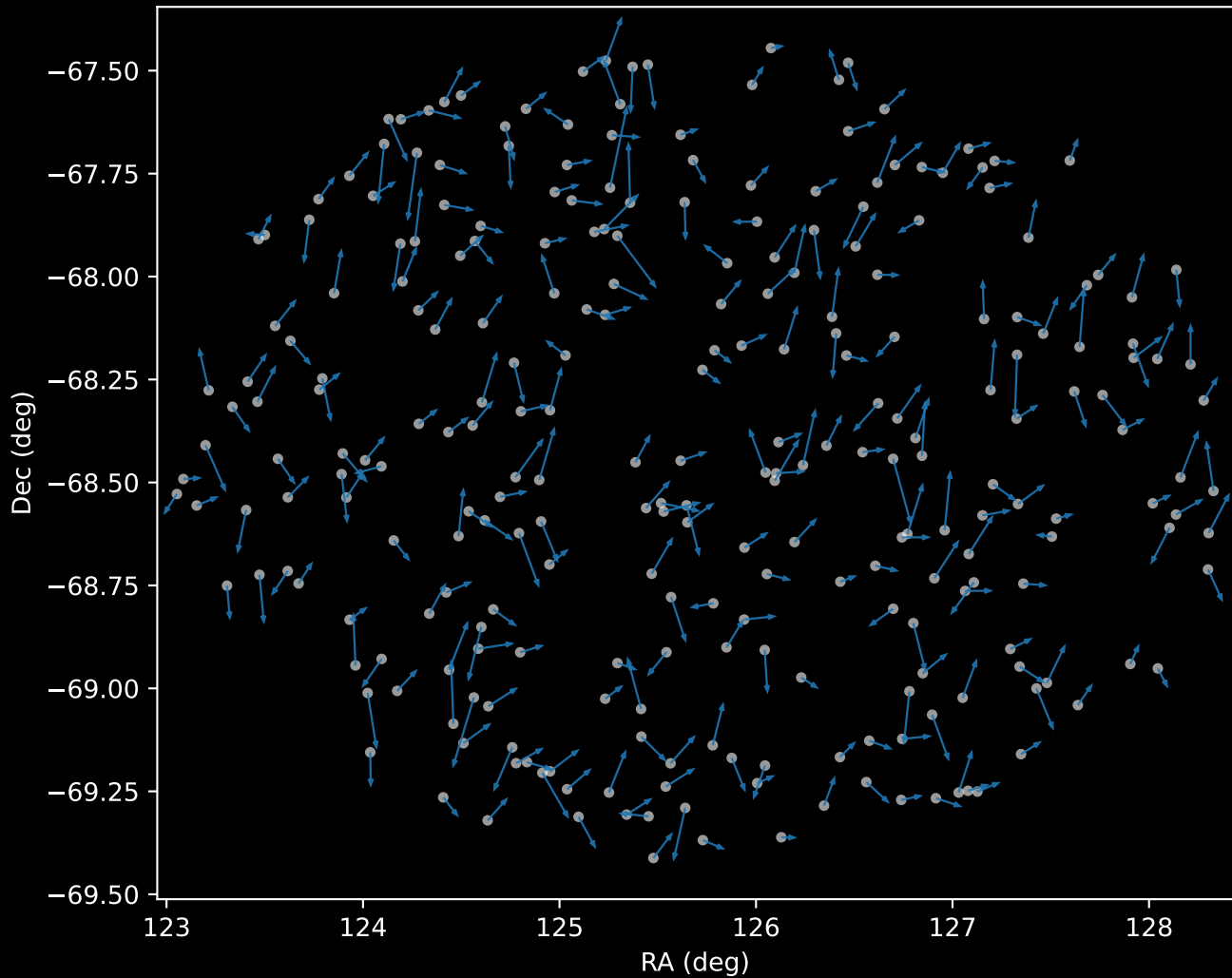
GALAH DR4 Cluster 0 Proper Motion Vectors (n=268)
