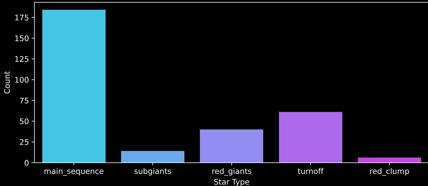
GALAH DR4 Field: [7045] Count plot of Star Type
