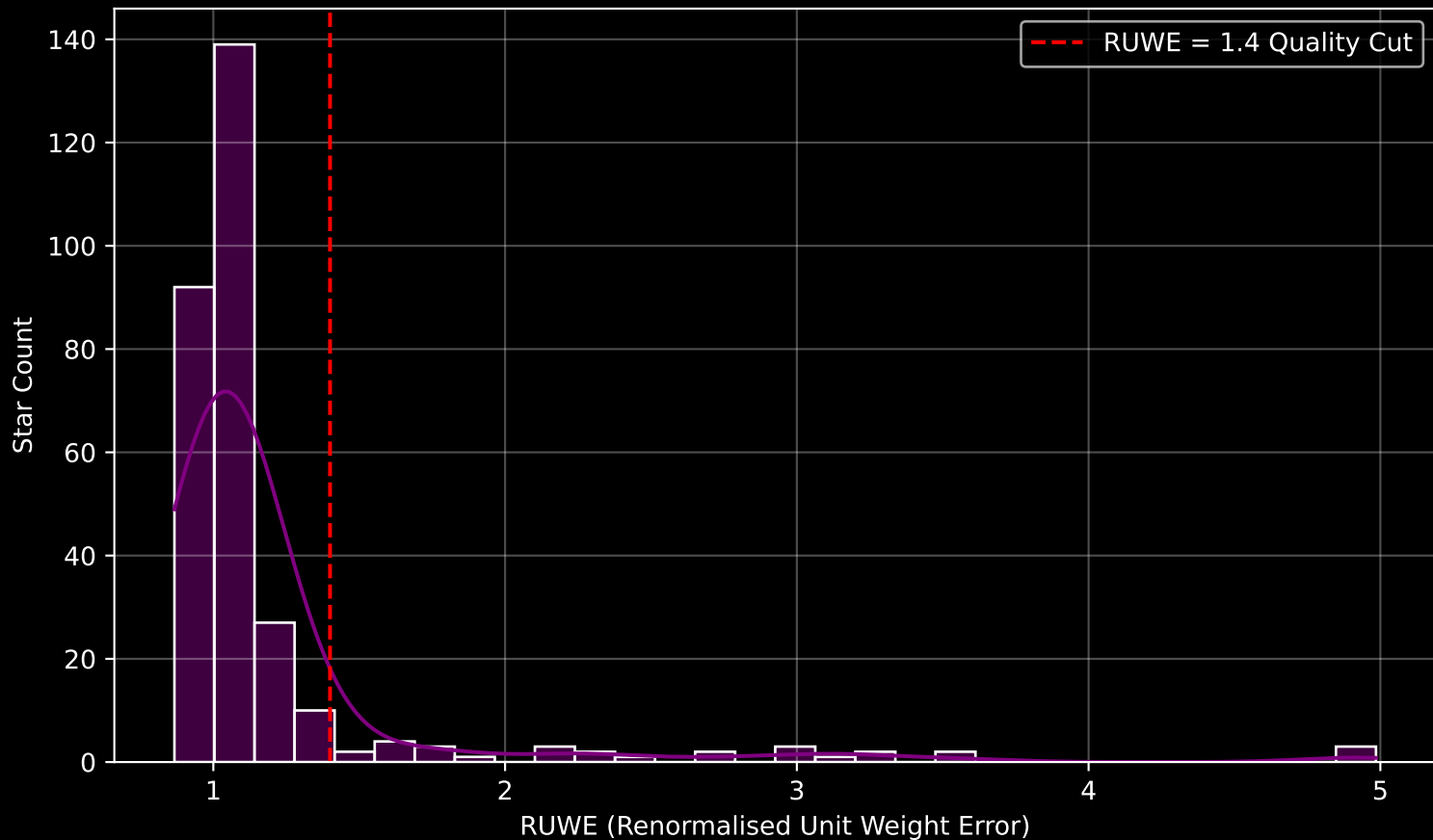
GALAH DR4 Field [7045] RUWE Distribution (n= 297)
