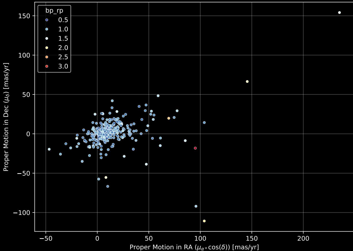
GALAH DR4 Field: [7045] Proper Motion Diagram (n= 305)
