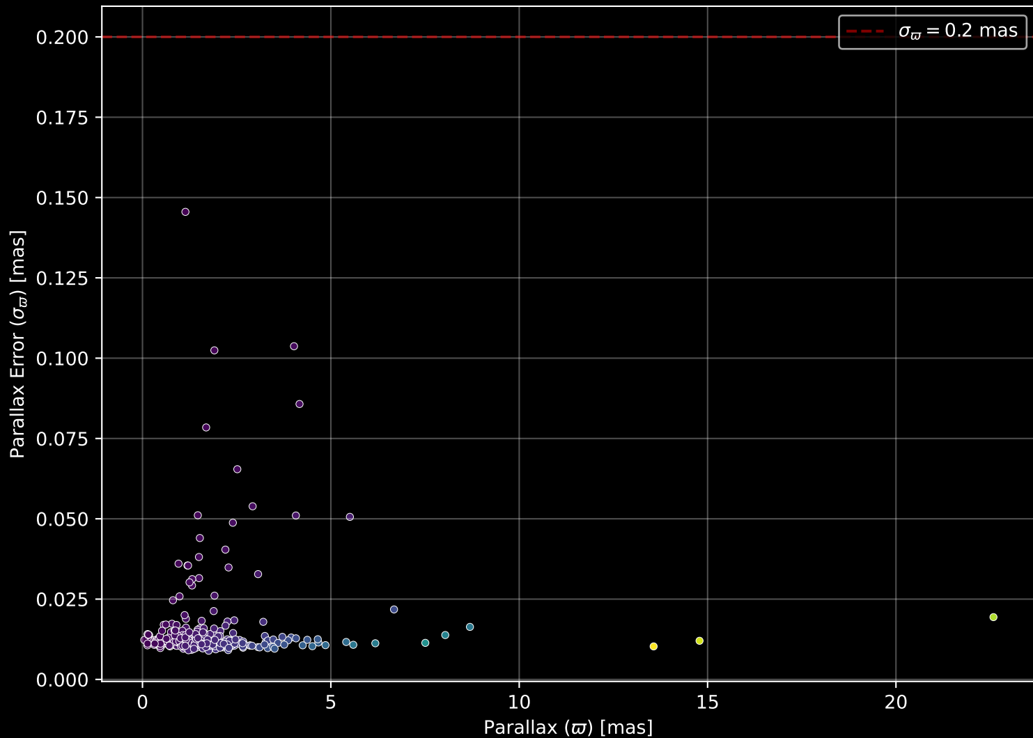
GALAH DR4 Field: [7045] Parallax Quality (n= 305)
